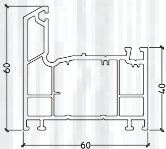
PB 201 CASEMENT FRAME (60*60)
