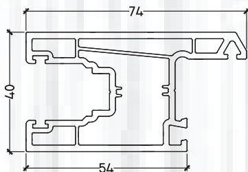
PB 107 SLIDING SASH WINDOW (74*40)
