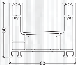
PB-101 SLIDING FRAME TWO TRACK
