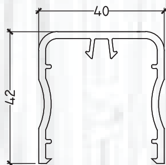
PB 404 HURRICANE BAR
