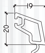
PB 114 SLIDING SINGLE GLAZING BEAD
