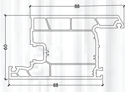
PB 206 CASEMENT DOOR SASH (INWARD)
