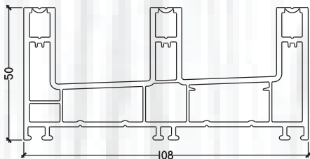
PB-104 SLIDING FRAME THREE TRACK
