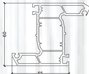
PB 209 CASEMENT Z-MULLION
