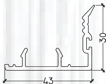
PB 110 SLIDING WINDOW INTERLOCK (43*30)
