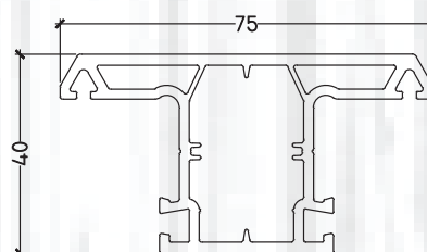
PB 119 MID RAIL SASH
