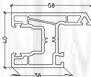
PB 105 SLIDING WINDOW SASH (58*40)
