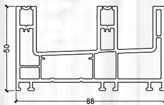
PB-102 2.5 TRACK SLIDER OUTER FRAME
