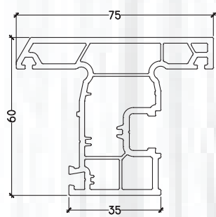
PB 205 CASEMENT WINDOW SASH (OUTWARD)
