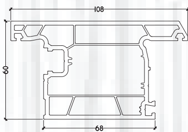
PB 207 CASEMENT DOOR SASH (OUTWARD)
