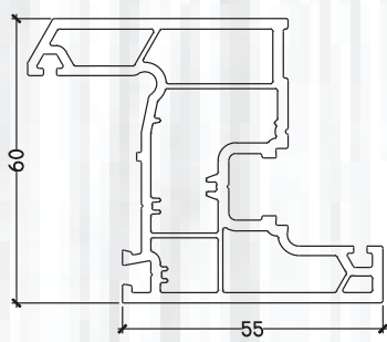
PB 204 CASEMENT WINDOW SASH (INWARD)
