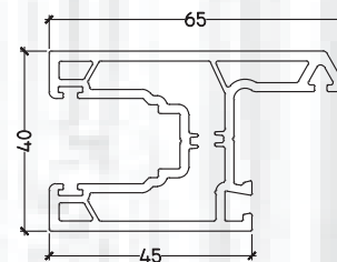
PB 106 SLIDING WINDOW SASH (65*40)
