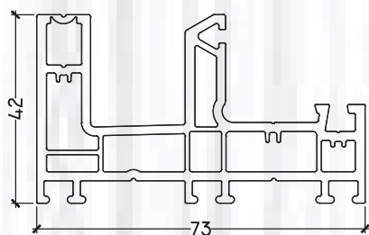
PB 118 MONO RAIL
