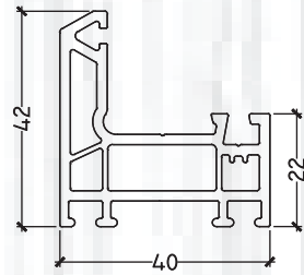
PB 203 CASEMENT NARROW FRAME (42*40)
