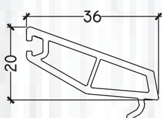
PB 211 CASEMENT SINGLE GLAZING BEAD
