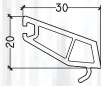
PB 212 CASEMENT DOUBLE GLAZING BEAD
