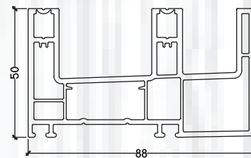
PB 103 2.5 TRACK SLIDER OUTER FRAME FLAT BOTTOM
