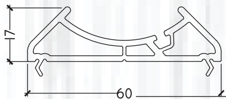
PB 402 ROUND POLL COUPLING
