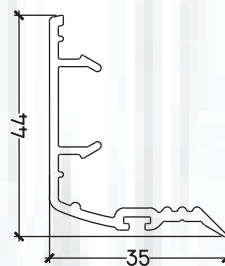
PB 111 SLIDING WINDOW INTERLOCK (44*35)
