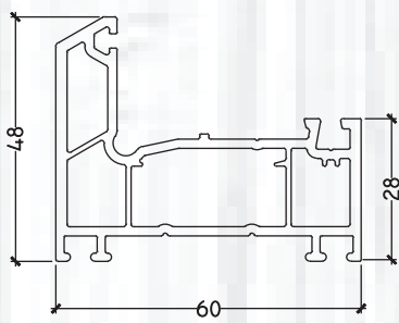
PB 202 SMALL CASEMENT FRAME (48*60)
