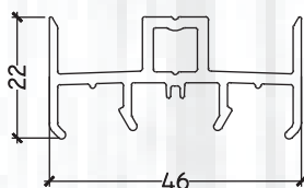
PB 116 MULTI PANE ADAPTER
