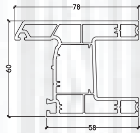
PB 213 CASEMENT SLIDING FIX FRAME
