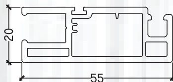
PB 113 FLYSCREEN SHASH
