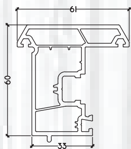
PB 210 FRENCH MULLION
